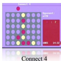
Connect 4
