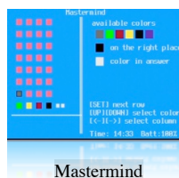
Mastermind
