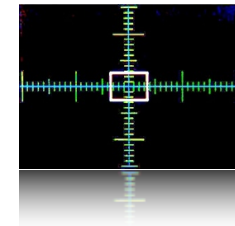
Rulers Grid
