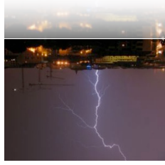
Motion Detect
