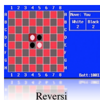
Reversi
